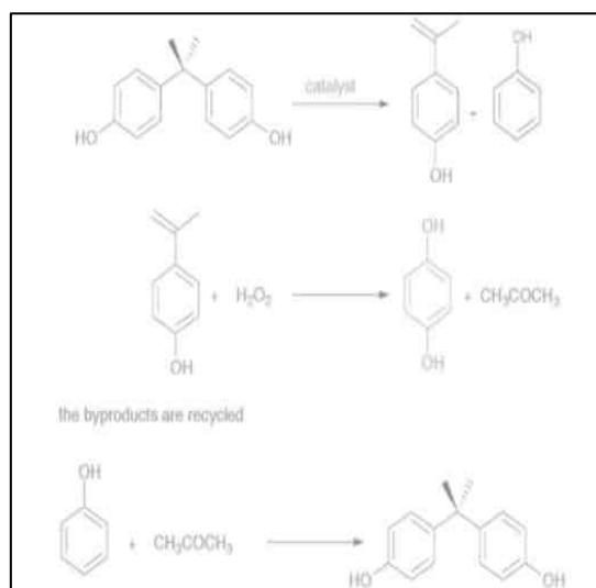
Fig 4: The New Upjohn Route to Hydroquinone
